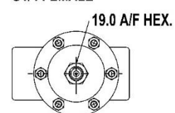
FEMALE CONNECTION
