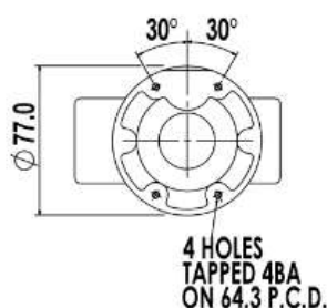
BLOCK BASE
